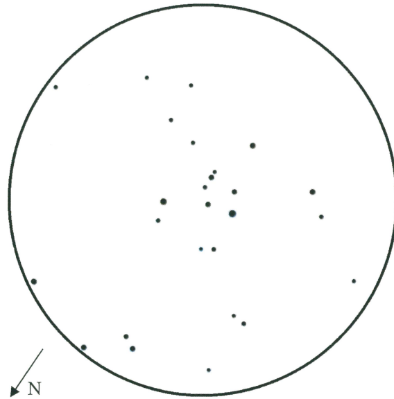
\delta Lyr
