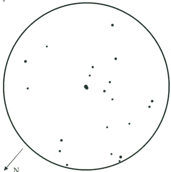
\beta Lyr
