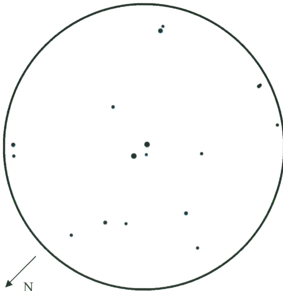
\epsilon Lyr
